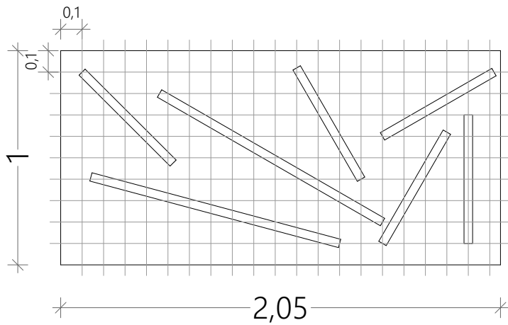
TYPE 1: T8 LED tubes of 120cm & 60cm
