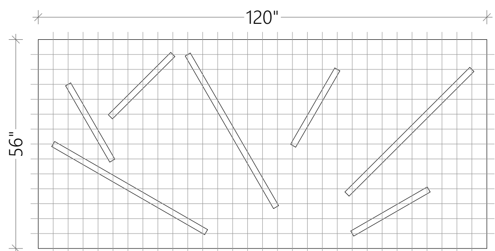
TYPE 3: T8 LED tubes 4' & 2'
