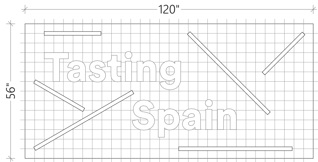
TYPE A: Backlit letters "Tasting Spain" Typography: Circular Black. Text height: 1'. T8 LED tubes 4' & 2'
