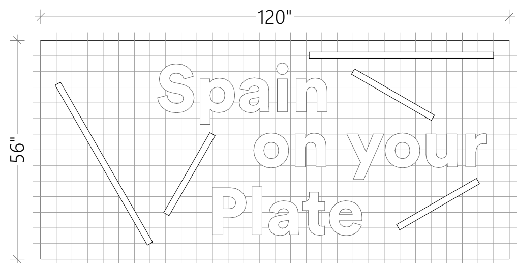
TYPE B: Backlit letters "Spain on your plate" Typography: Circular Black. Text height: 1'. T8 LED tubes 4' & 2'
