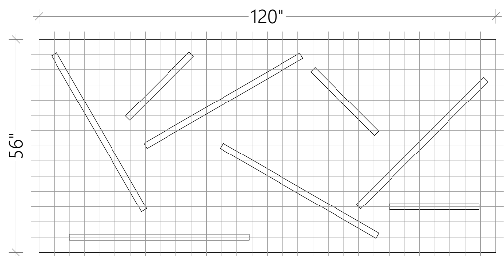
TYPE 2: T8 LED tubes 4' & 2'
